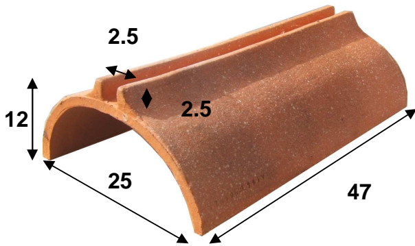
FAITIERE A GORGE FF50 2.1 PCS/ML
